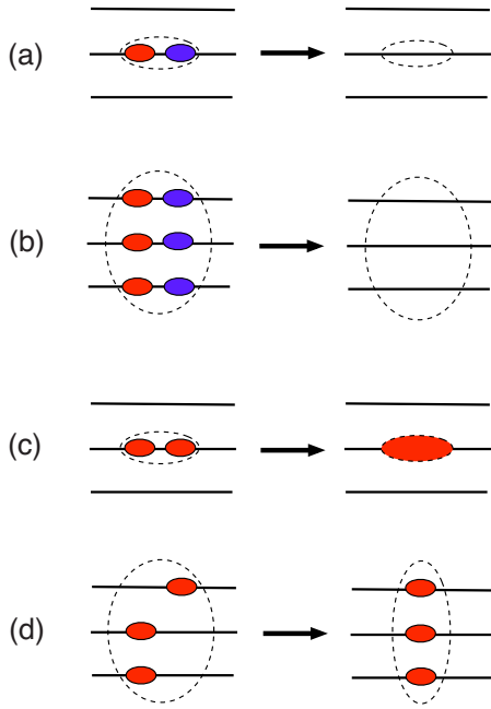
FIG. 1. (Color online) Pictorial summary of the renormalization group procedure discussed in Appendixes B and C. If an object and its antioobject are very closely spaced, then they will cancel upon coarse graining, but in the process the coupling constants will be renormalized. (a) shows the simplest such process involving single pancakes which may be viewed as integrating out the smallest loops of magnetic flux. (b) is an example of the more complicated object/antioobject cancellations which correspond to integrating out larger loops. Nearby objects that are not antiparticles will fuse together. (c) shows two single strength pancakes fusing into a double strength pancake. (d) shows a height two stack and a single pancake fusing into a height three stack.
