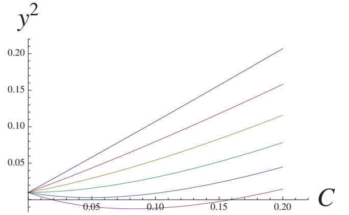
FIG. 2. (Color online) Plot of the flow trajectories of Eq. (3.13) for the case where the initial fugacity y_0=0.1 . The six curves, from top to bottom, are for \beta q^2=1-6 , respectively. Since the flow stops when y=0 , this initial condition implies a phase transition occurring for \beta q^2 between 5 and 6.
